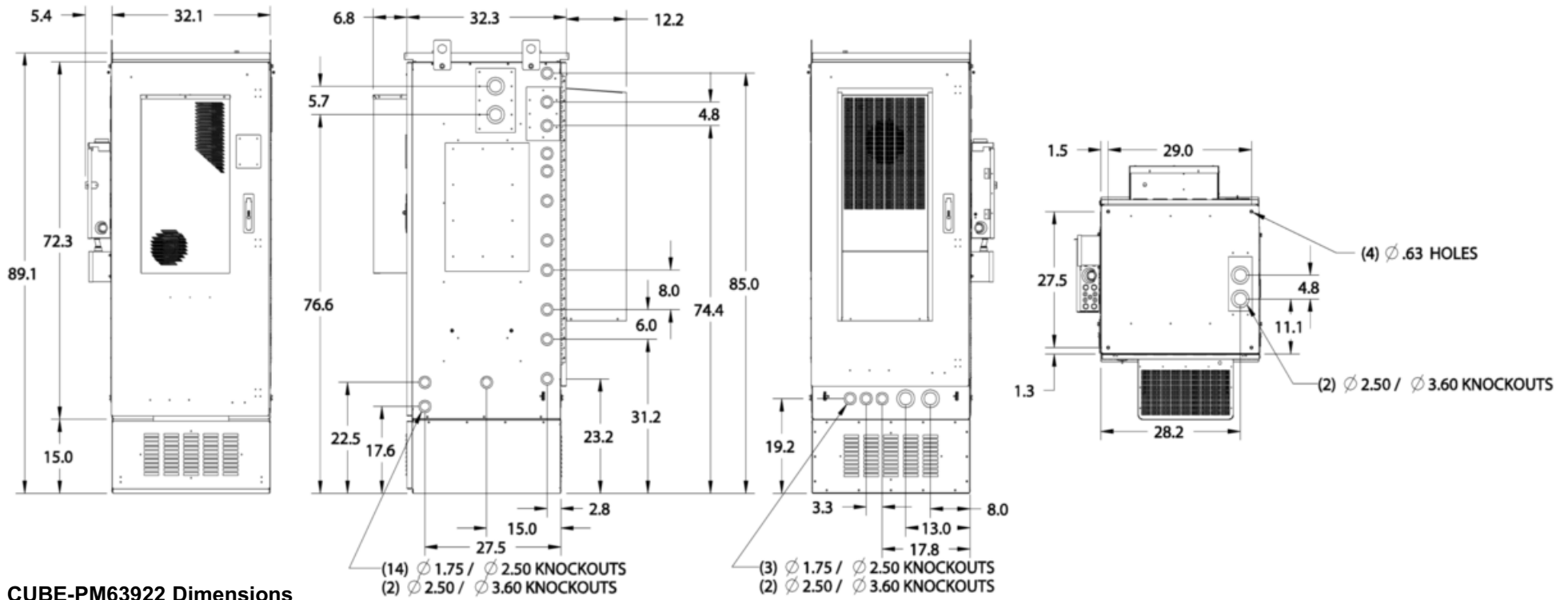
CUBE-PM63922 Dimensions (All units in inches)
